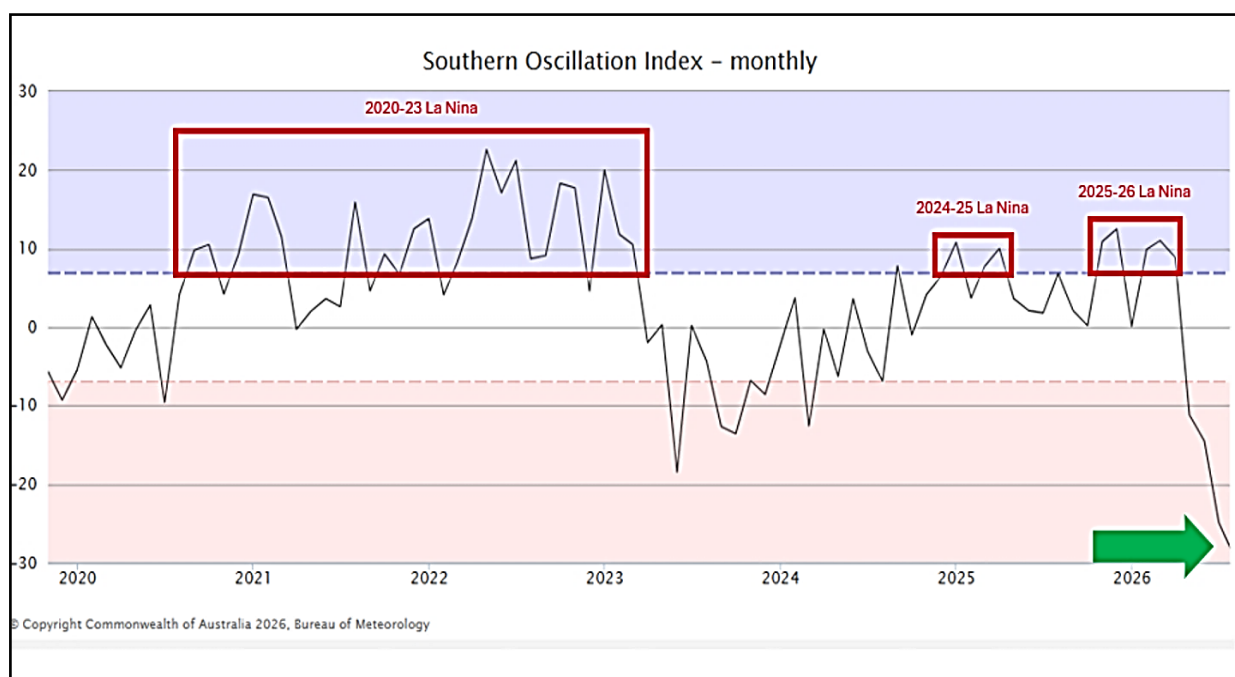
Figure 1 - Southern Oscillation Index (SOI) – monthly history with recent La Niña events indicated.
