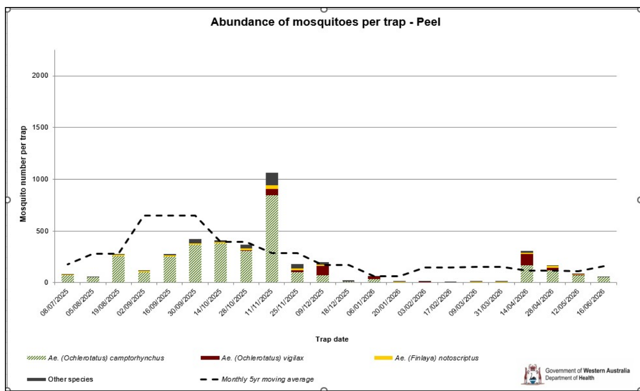
Figure 10. - WA Department of Health - Peel average trap abundance July 2025 – June 2026 Source: Medical Entomology Branch, WA Department of Health - Medical Entomology
