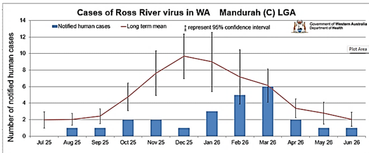
Figure 11. - Ross River virus Mandurah 2025/2026. Source: Medical Entomology Branch, WA Department of Health
