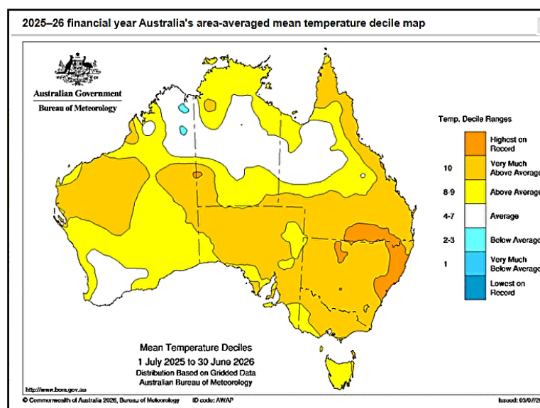
Figure 5. - 2025/26 Australian area averaged mean temperature compared to historical records. Source - Australian Government Bureau of Meteorology/Financial year climate and water statement 2025/26. Water Level Observations
