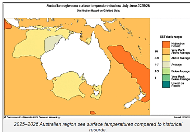
Figure 4. - 2025/26 Australian region sea surface temperatures compared to historical records. Source - Australian Government Bureau of Meteorology/Financial year climate and water statement 2025/26.
